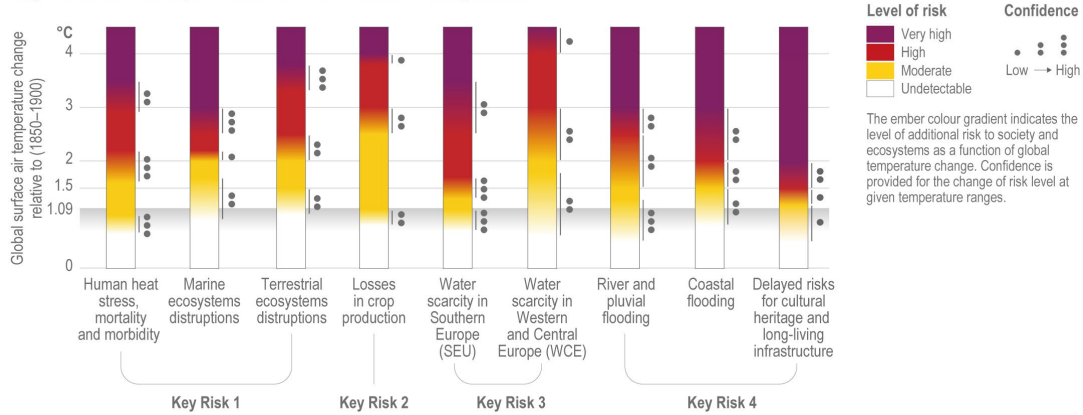
Figure 2: Burning ember diagrams for key risks for Europe under low to medium adaptation. {Figure 13.28}
