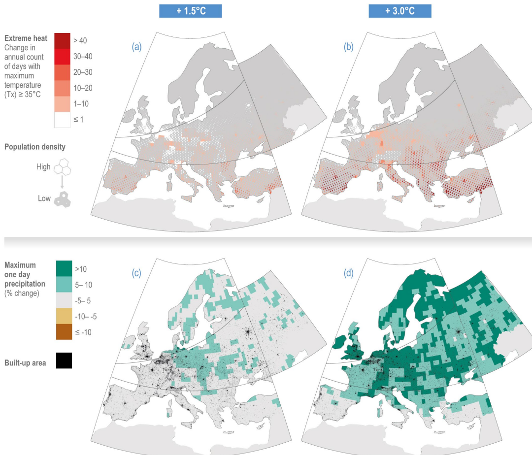
Figure 1: Changes in climate hazards for global warming levels of 1.5°C and 3°C based on the CMIP6 ensemble with respect to the baseline period 1995-2014, combined with information on present exposure or vulnerability.
